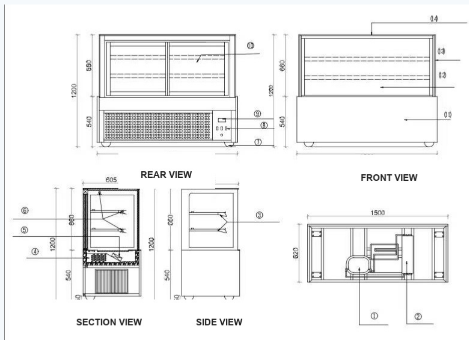
DIMENSION DRAWING - NOT TO SCALE
