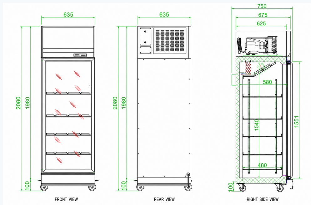
DIMENSION DRAWING - NOT TO SCALE
